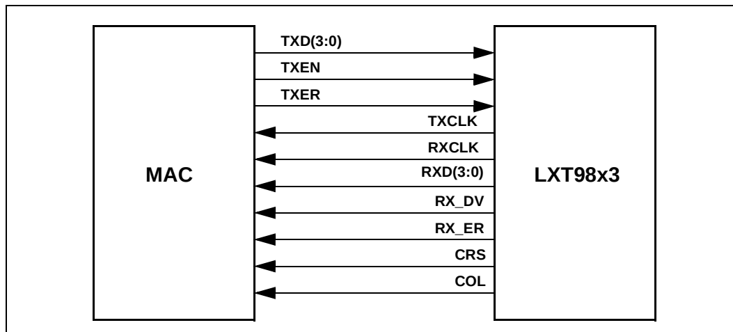
Figure 4. MII Interface
