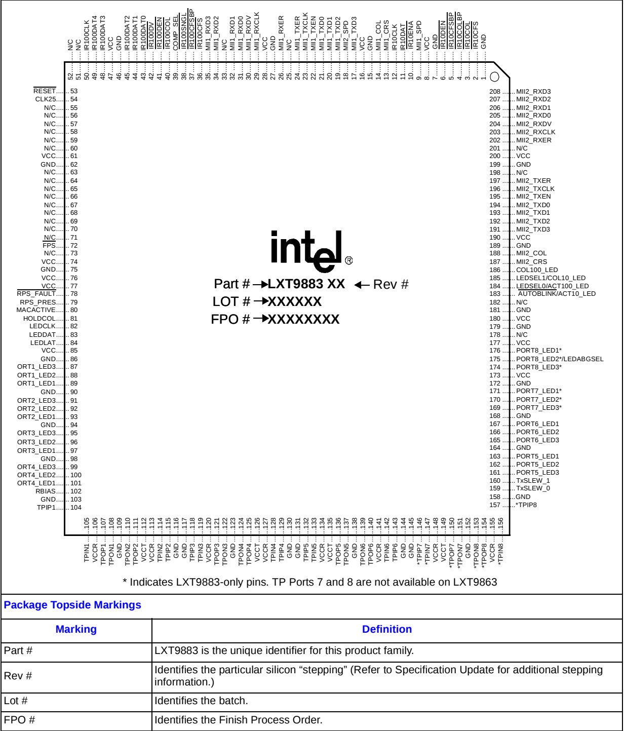
Figure 2. LXT9883 Pin Assignments
