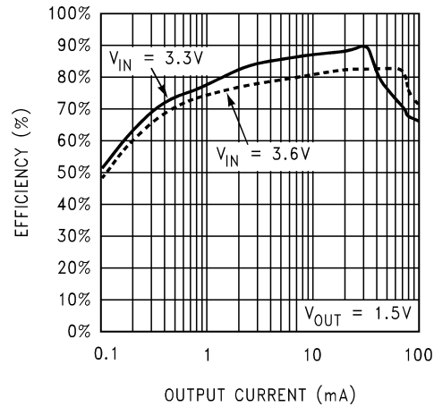
Efficiency vs. Output Current: LM2798-1.5
