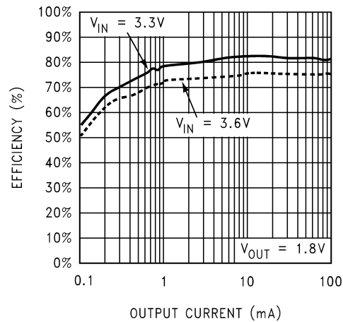
Efficiency vs. Output Current: LM2797/98-1.8
