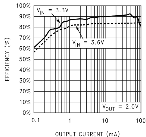
Efficiency vs. Output Current: LM2798-2.0
