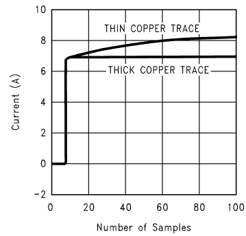
FIGURE 7. Transient Response to 7 Amp Step Current
