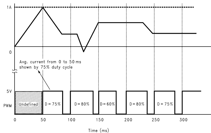
FIGURE 9. Typical Timing Diagram for Mostly Positive Current
