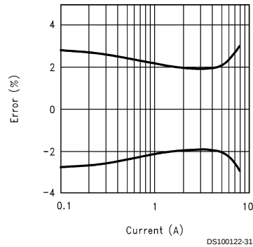
Error vs Current (LM3812-7.0 and LM3813-7.0) (Note 10)
