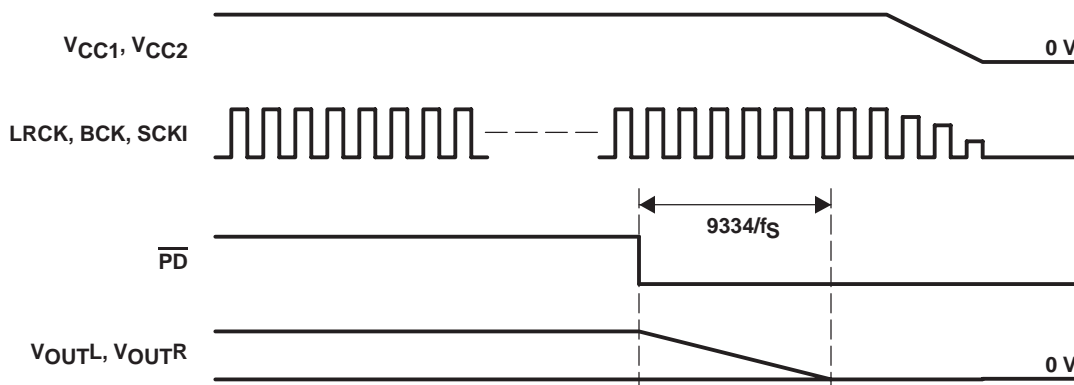
Figure 20. Power-Off Sequence
