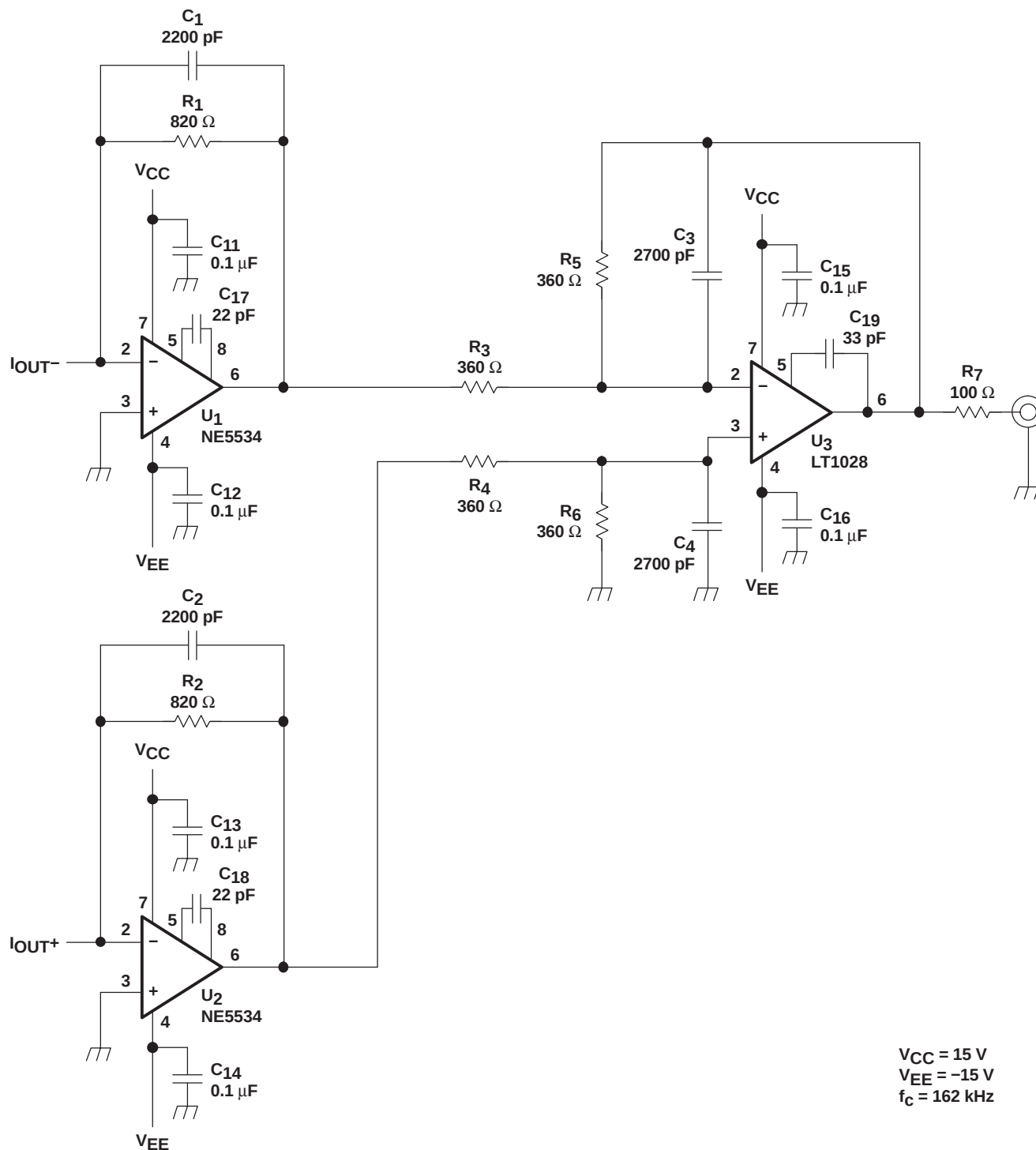
Figure 37. Measurement Circuit for PCM, V_{OUT} = 4.5 V rms
