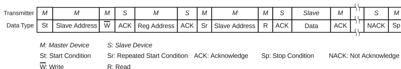
Figure 34. Read Operation
