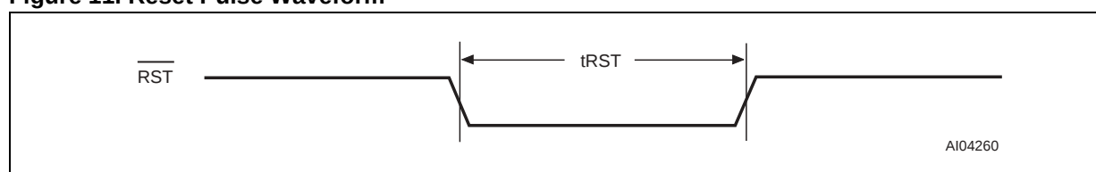
Figure 11. Reset Pulse Waveform
