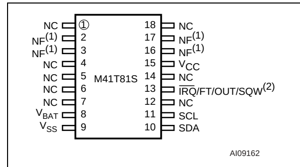
Figure 4. 18-pin, 300mil SOIC (MY) Connections
