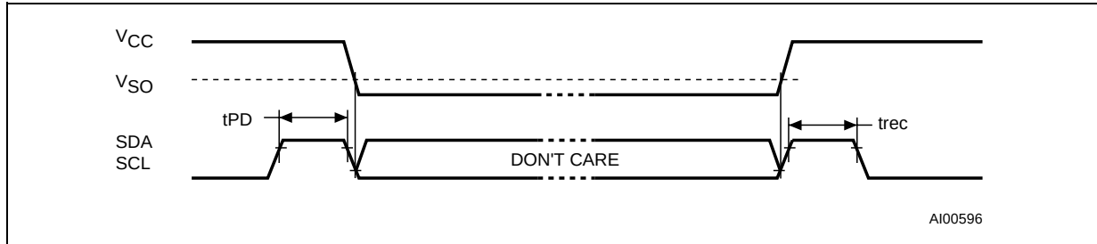
Figure 17. Power Down/Up Mode AC Waveforms
