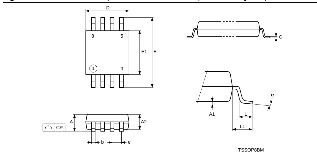
Figure 13. TSSOP8 – 8-lead, thin shrink small outline, 3x3mm body size, outline
