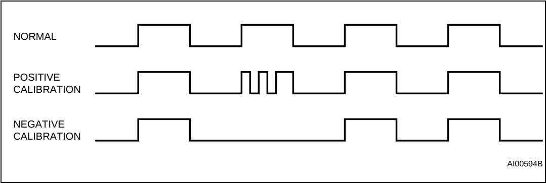
Figure 13. Clock calibration
