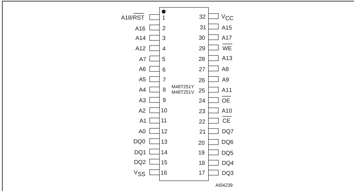
Figure 3. DIP Connections
