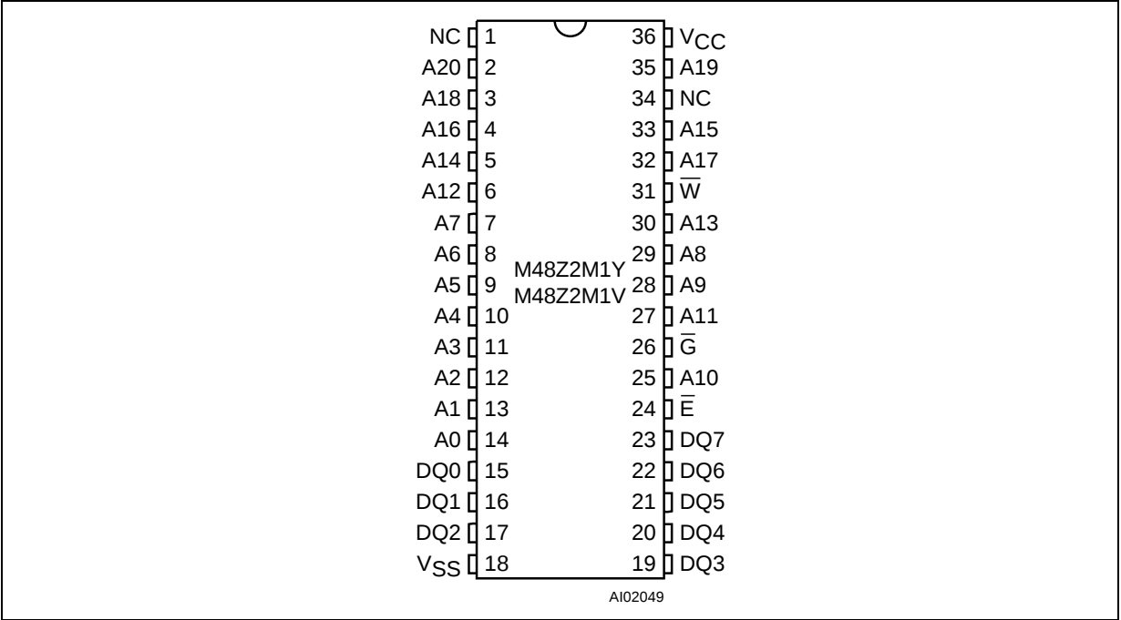
Figure 3. DIP Connections
