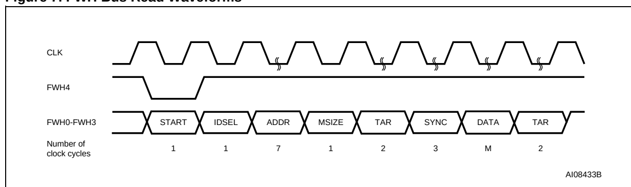
Figure 7. FWH Bus Read Waveforms
