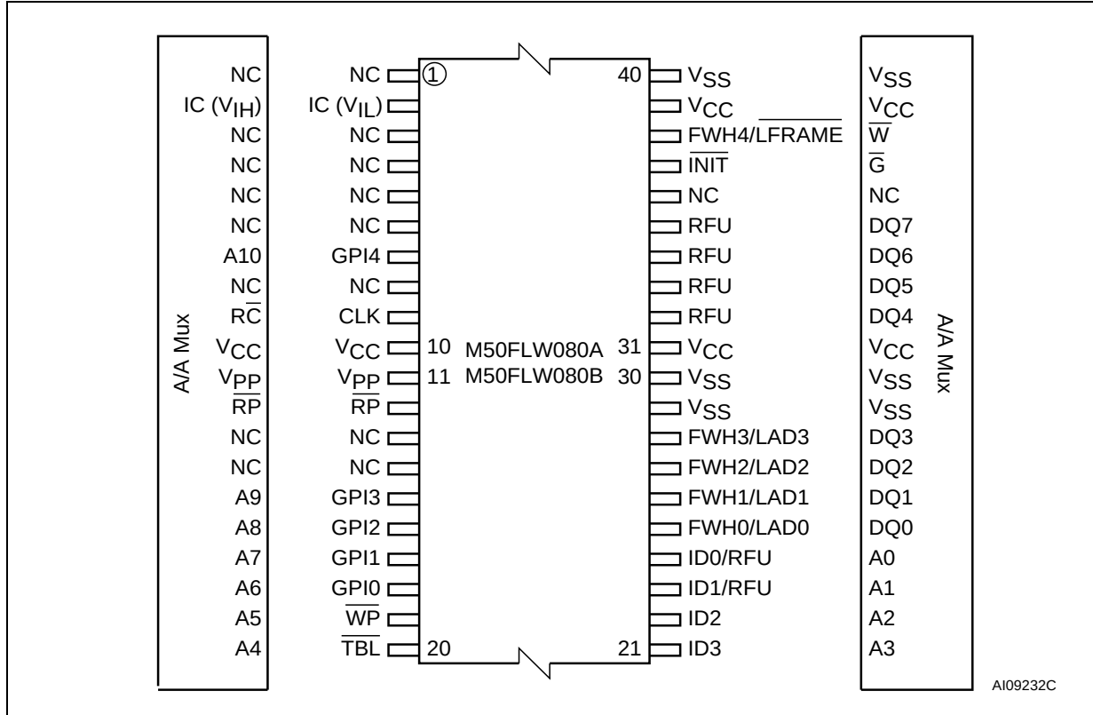
Figure 6. TSOP40 Connections
