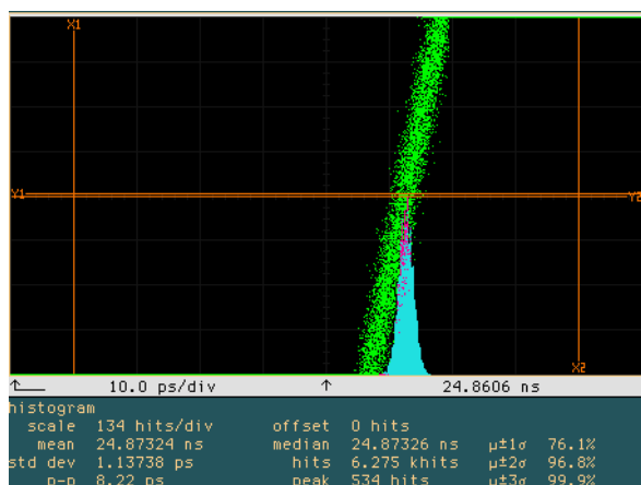
Figure 5: Broadband Jitter
