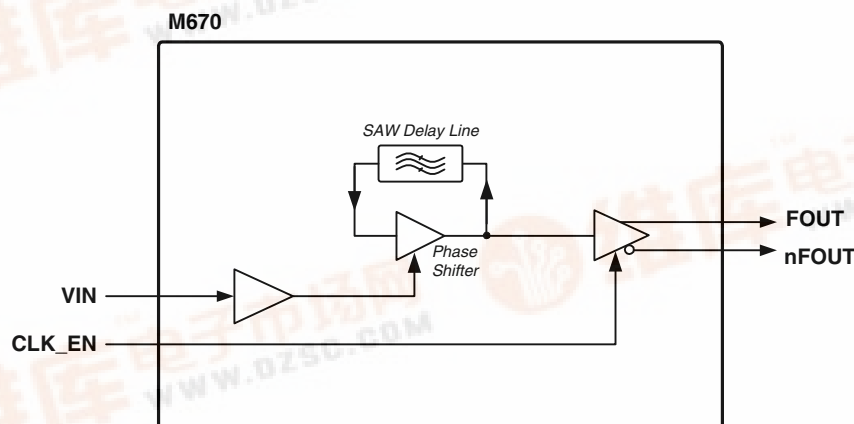
Figure 2: Block Diagram
