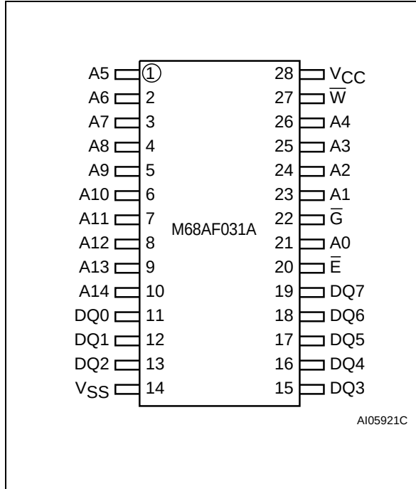
Figure 3. SO Connections
