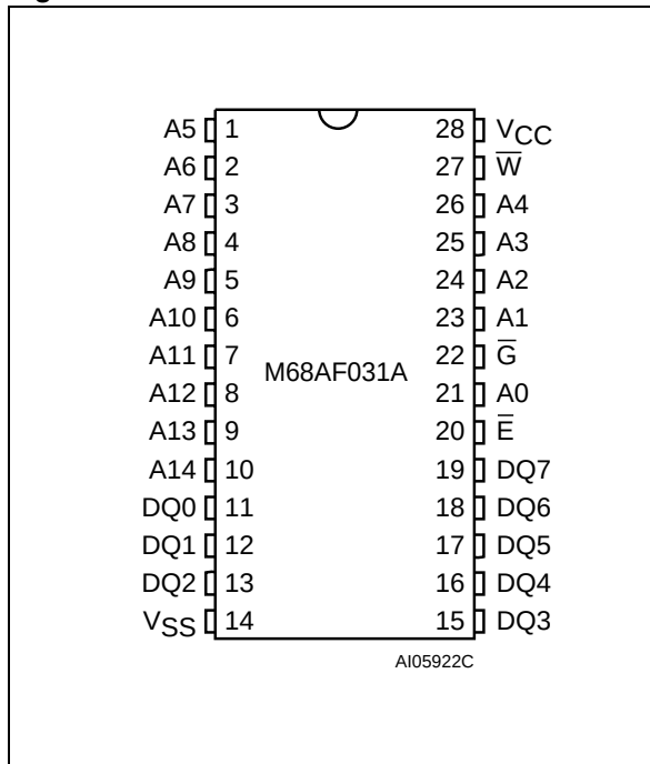
Figure 4. DIP Connections
