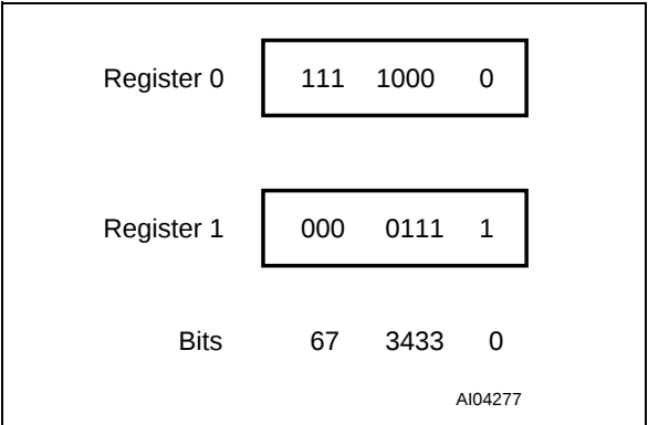
Figure 15. Global Mask Register Patterns
