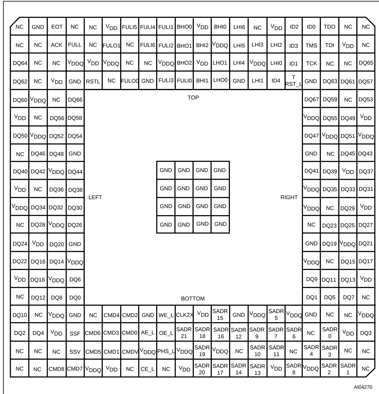
Figure 3. Connections
