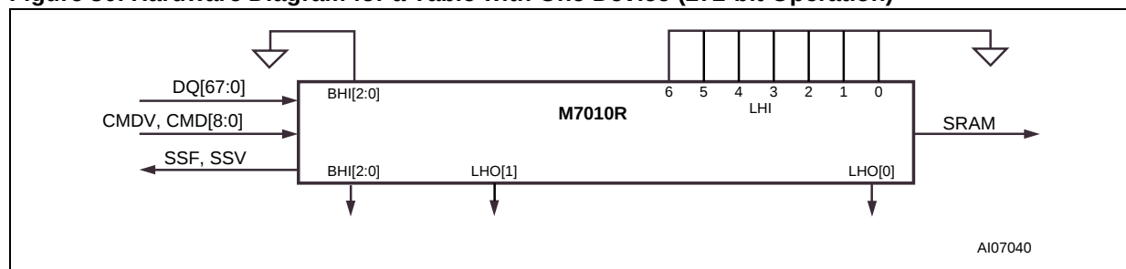
Figure 30. Hardware Diagram for a Table with One Device (272-bit Operation)
