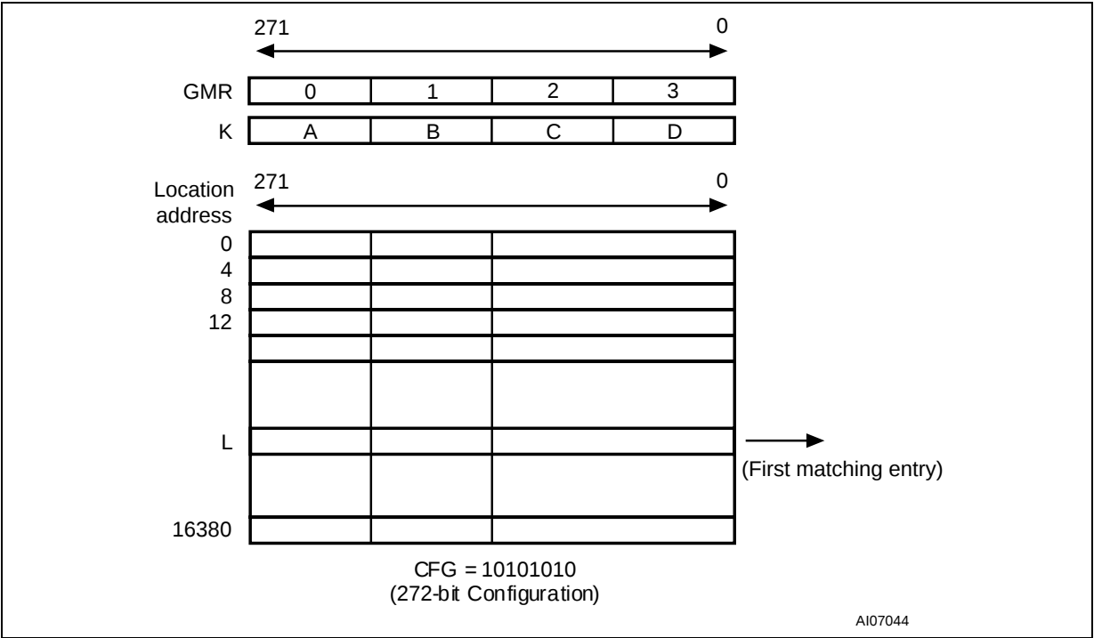
Figure 32. x272 Table with One Device
