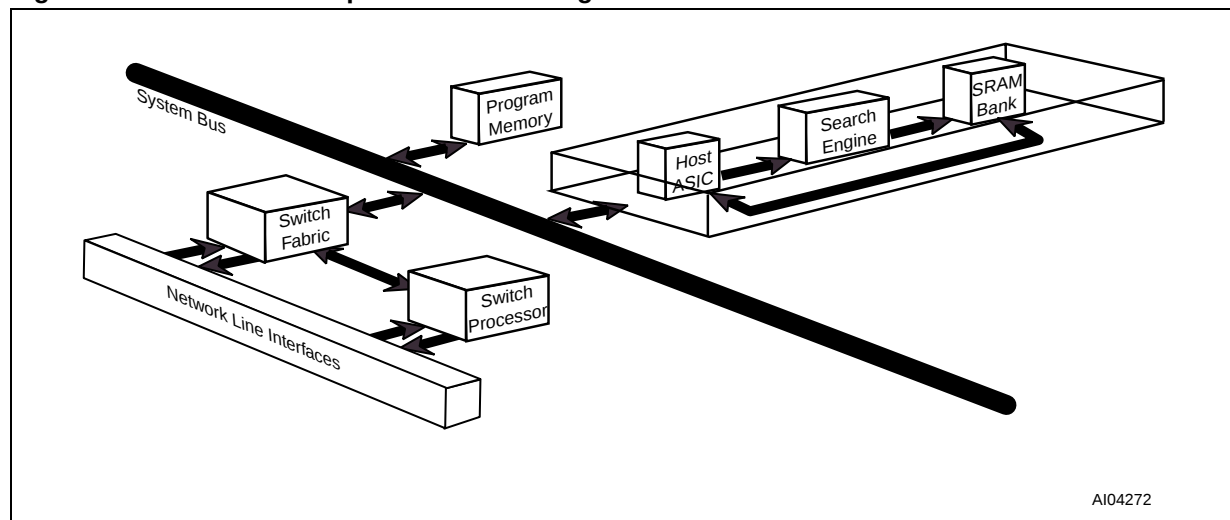
Figure 2. Switch/Router Implementation Using the M7010R
