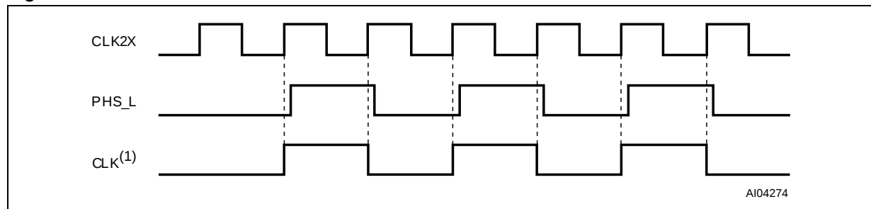
Figure 12. Clocks
