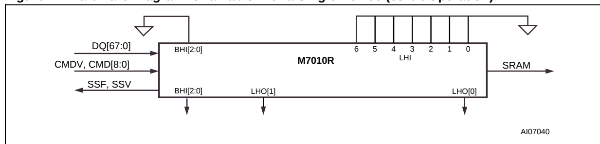
Figure 24. Hardware Diagram for a Table with a Single Device (68-bit Operation)
