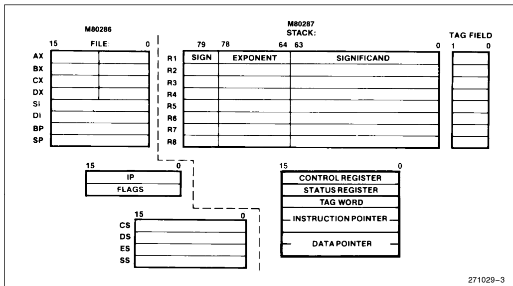
Figure 3. M80286/20 Architecture
