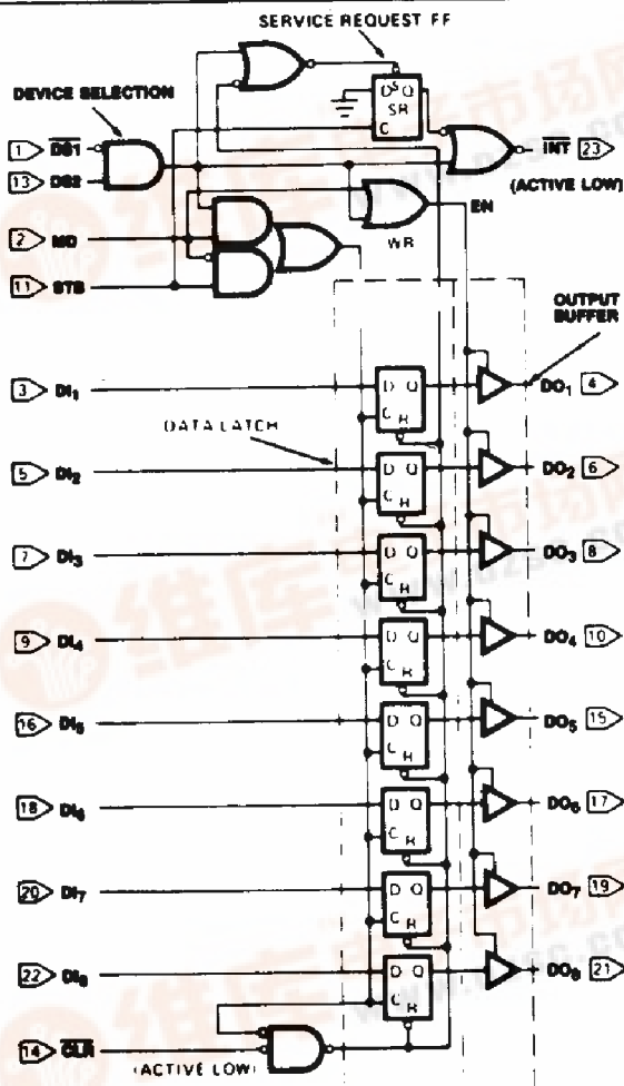
Figure 1. Logic Diagram
