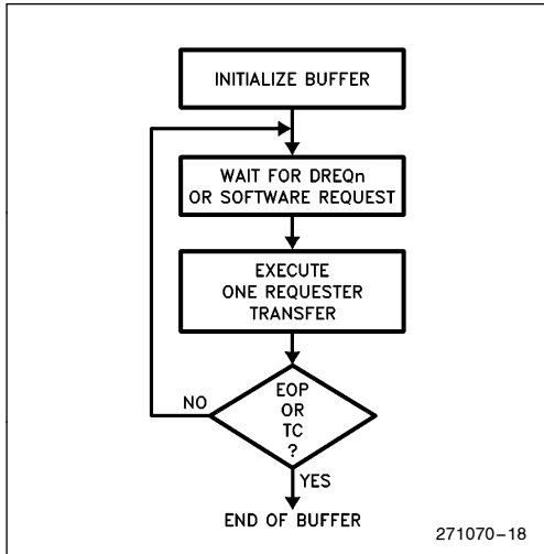
Figure 17. Buffer Transfer in Single Transfer Mode
