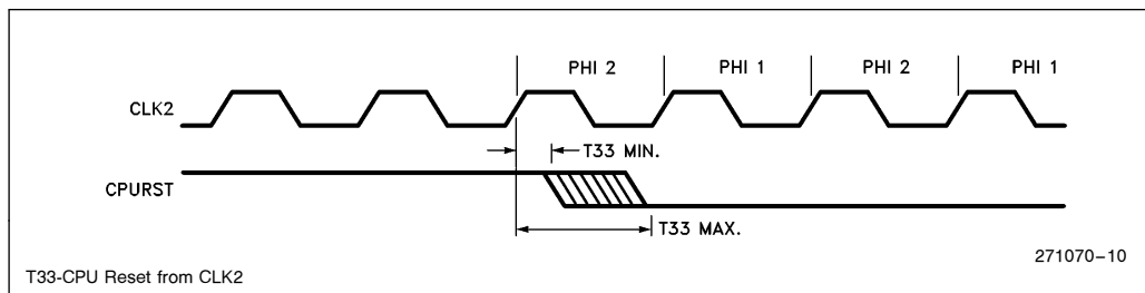
Figure 9. CPURST Timing
