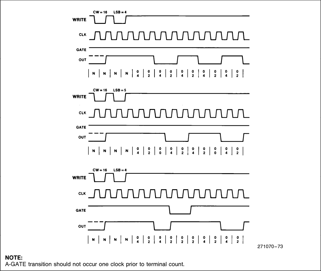
Figure 46. Mode 3
