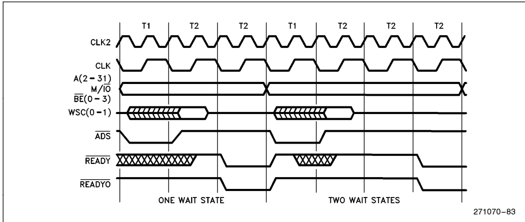
Figure 50. Wait States in Non-Pipelined Cycles
