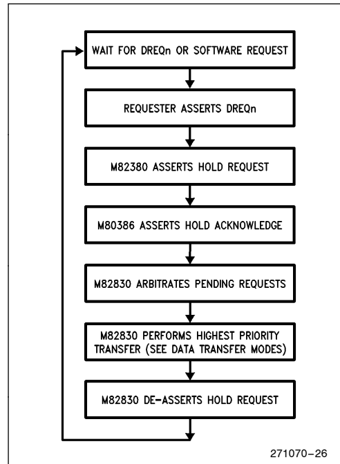
Figure 27. Bus Arbitration and DMA Sequence
