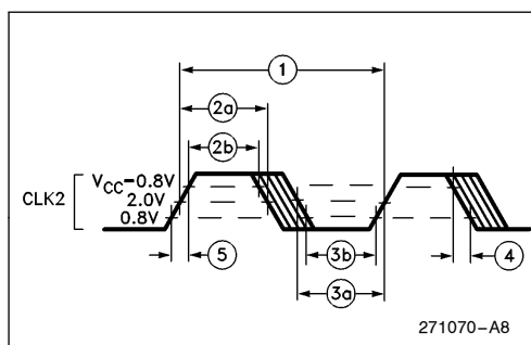
Figure 67. CLK2 Timing
