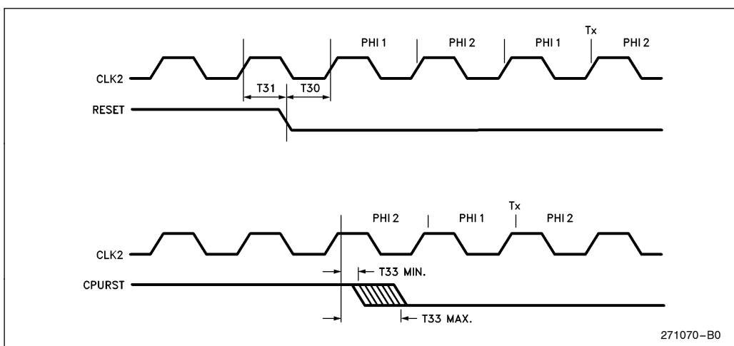
Figure 69. Reset Timing
