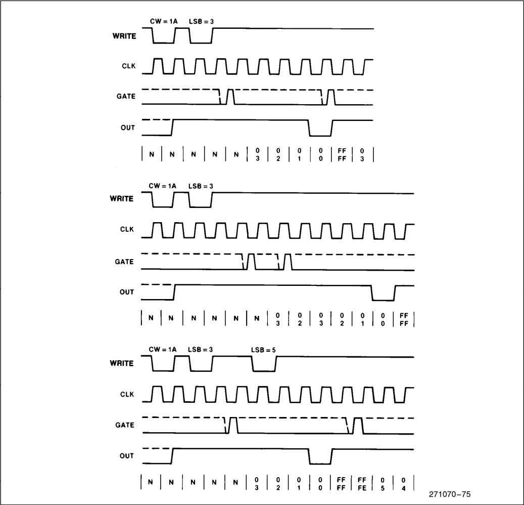
Figure 48. Mode 5
