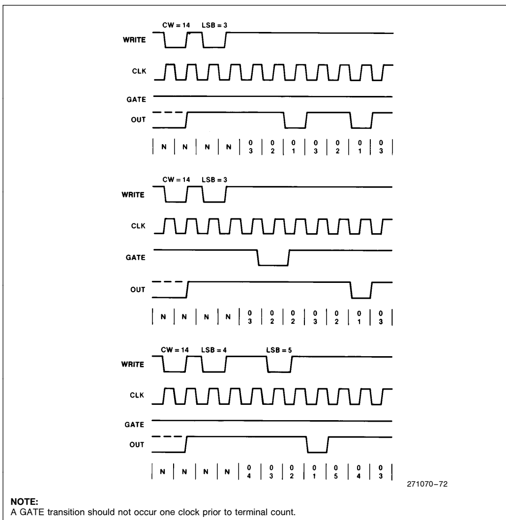
Figure 45. Mode 2
