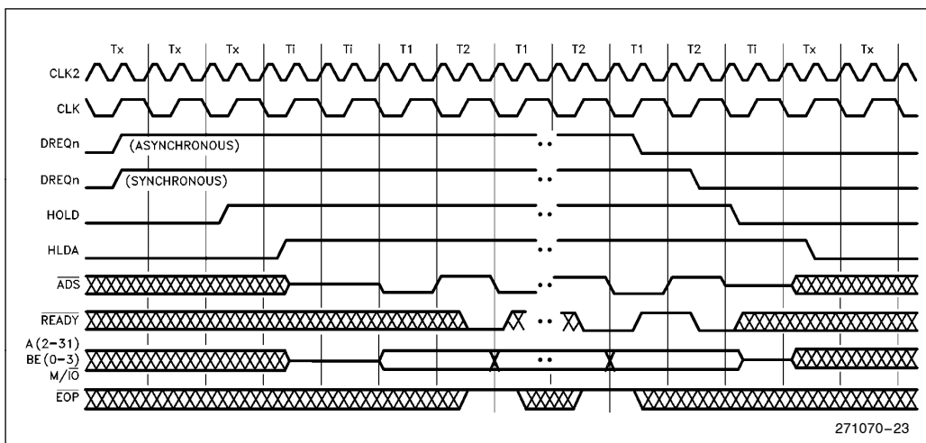
Figure 22. Demand Mode Transfers
