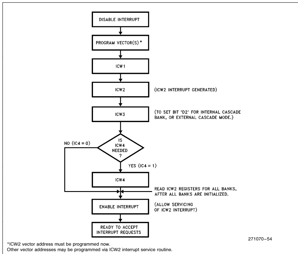
Figure 42. Initialization Sequence
