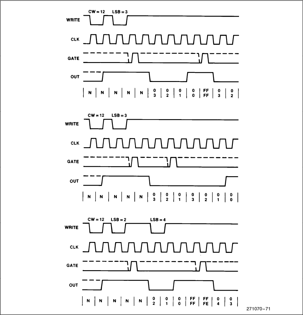
Figure 44. Mode 1
