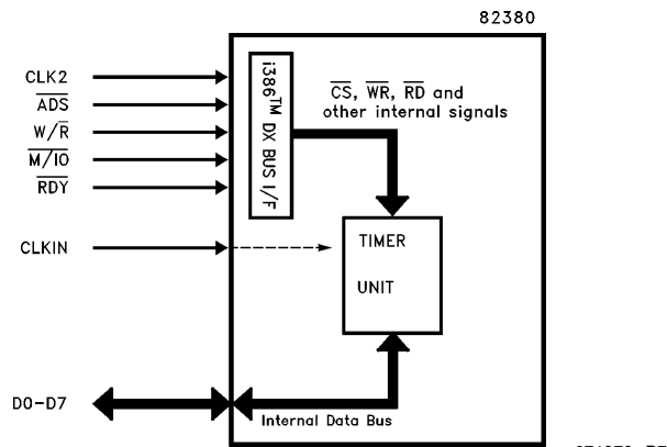
Figure 1. Translation of i386™ DX Signals to Internal M82380 Timer Unit Signals
