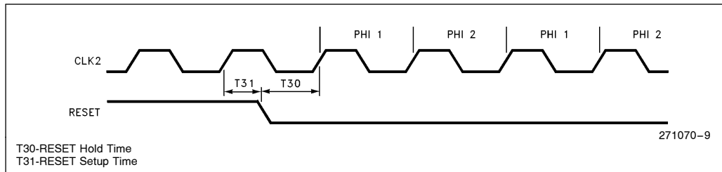
Figure 8. RESET Timing
