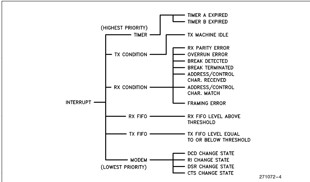
Figure 4. Interrupt Structure
