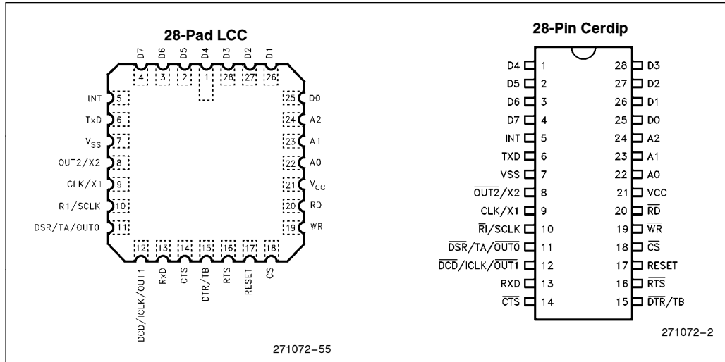
Figure 2. Package Pinouts
