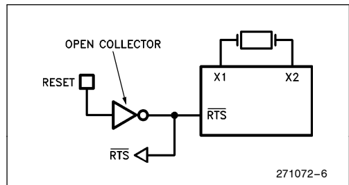
Figure 6. Strapping Option
