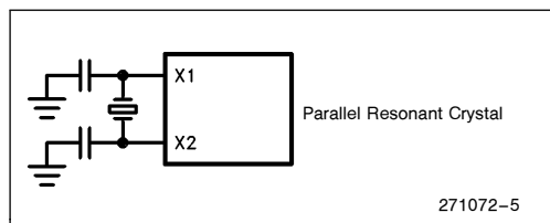
Figure 5. Crystal Oscillator
