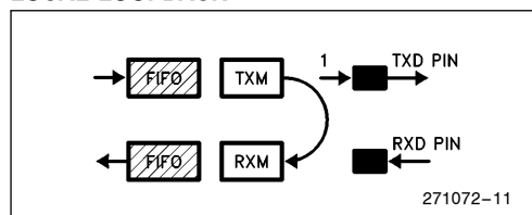
Figure 12. Local Loopback
