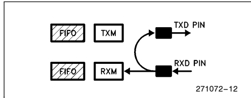
Figure 13. Remote Loopback
