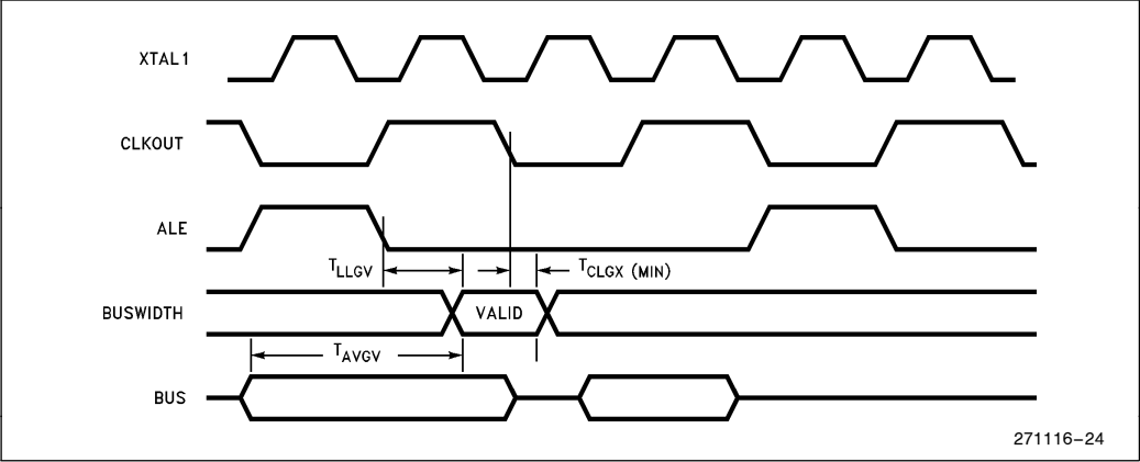
Figure 8. Buswidth Timings
