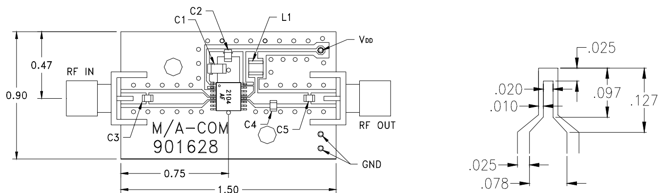
Top view
