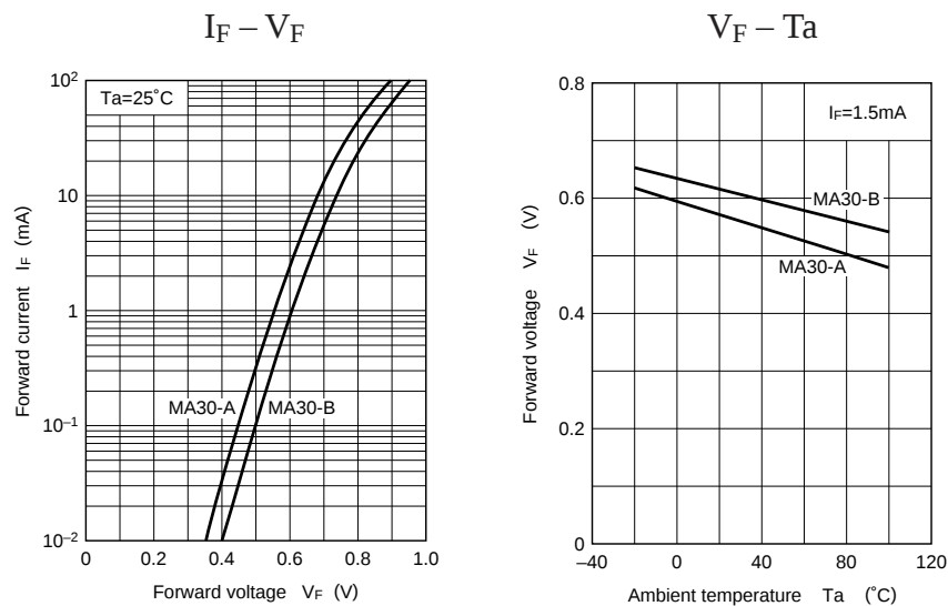
Characteristics chart of MA30W
