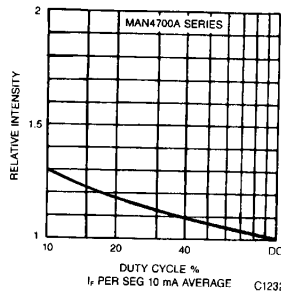
Fig. 13. Relative Luminous Intensity vs. Duty Cycle
