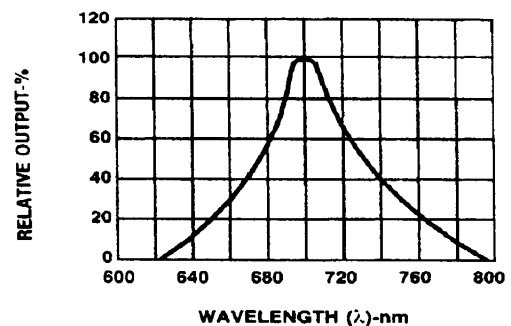
Fig.2 SPECTRAL RESPONSE
