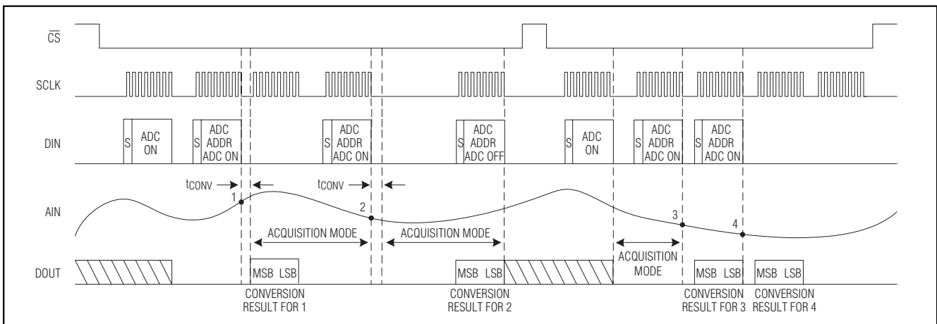
Figure 6. ADC Single Conversion Mode Timing Diagram
