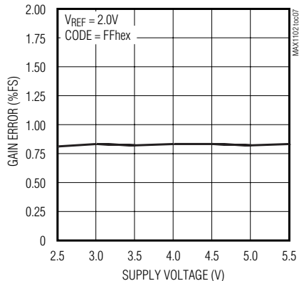
ADC GAIN ERROR vs. SUPPLY VOLTAGE
