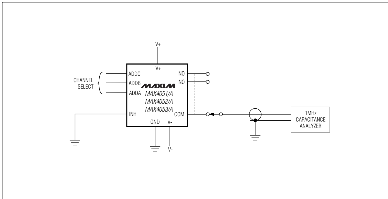
Figure 7. NO/COM Capacitance
