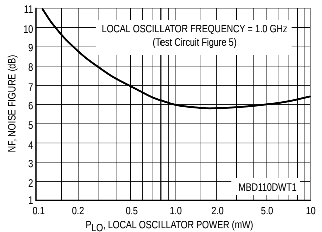
Figure 4. Noise Figure
