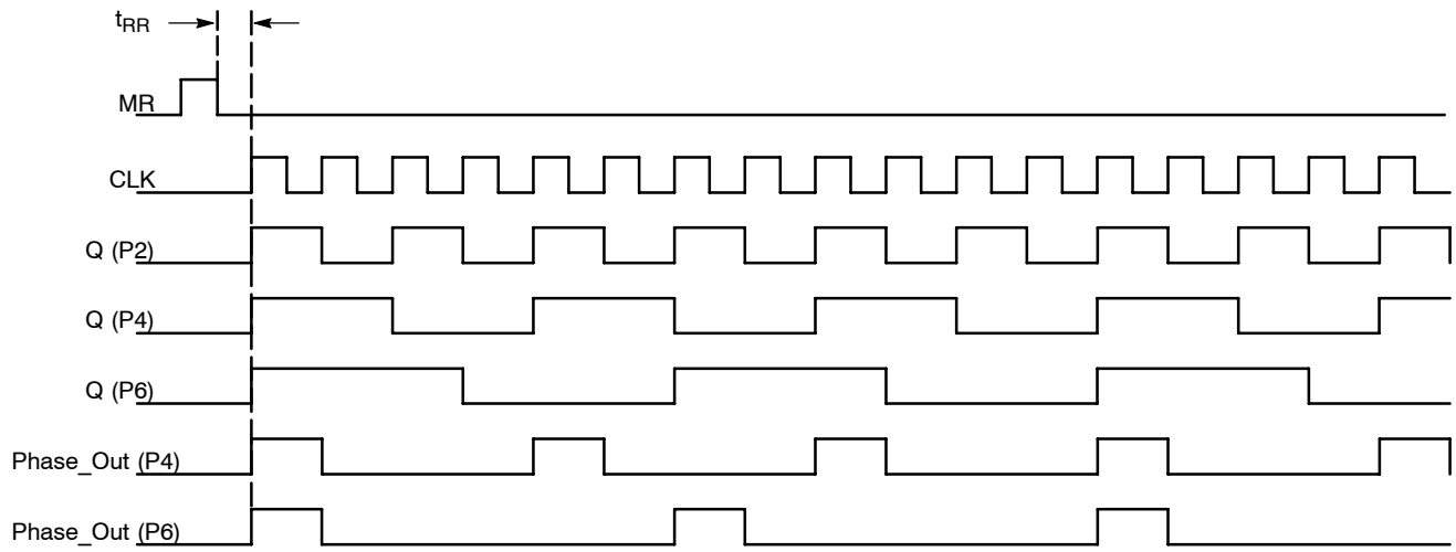
Figure 3. Timing Diagram
