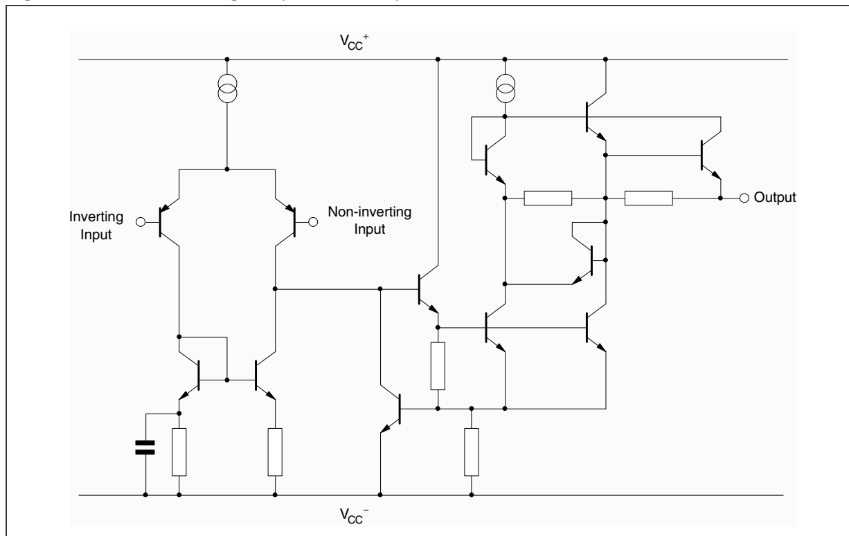
Figure 1. Schematic diagram (1/2 MC33078)
