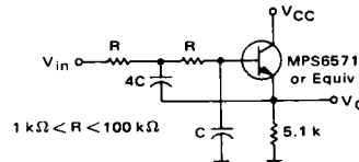
FIGURE 21 — EMITTER FOLLOWER LOW PASS FILTER
