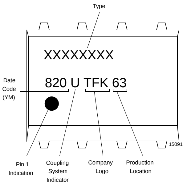
Figure 12. Marking example
