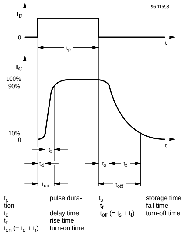
Figure 2. Switching times
