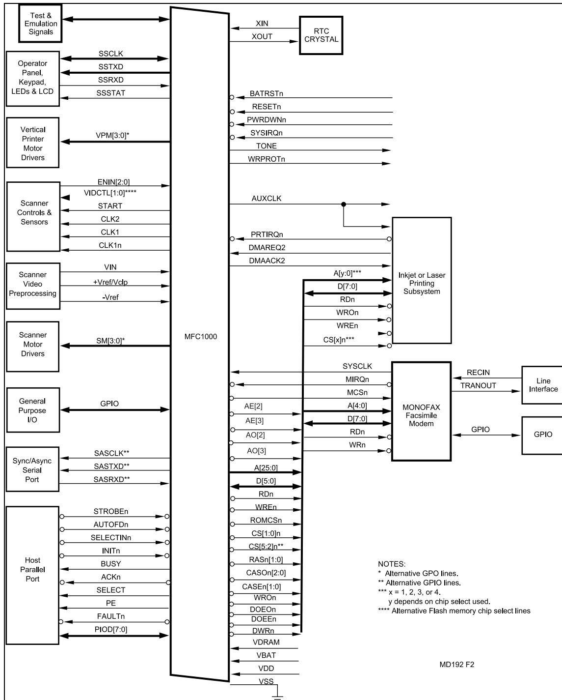
Figure 2. MFC1000 Controller Organization
