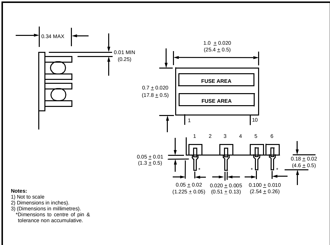
Figure 4 - Mechanical Data
