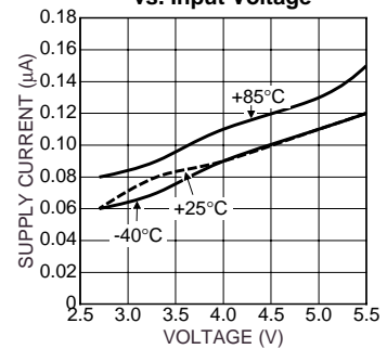
Supply Off Current vs. Input Voltage
