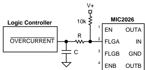
Figure 4. Transient Filter
