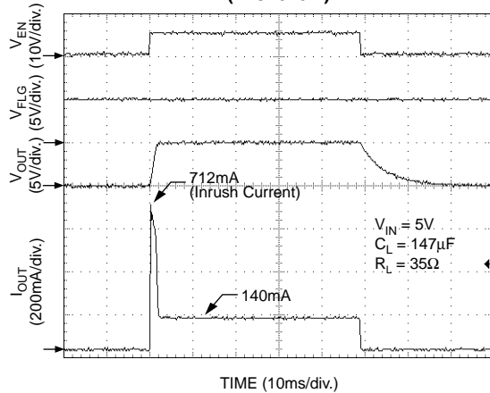
Turn-On/Turnoff (MIC2026-1)
