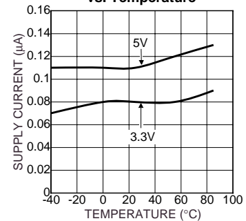
Supply Off Current vs. Temperature
