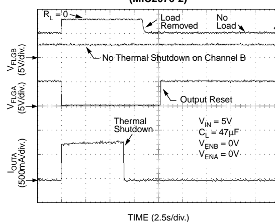
Independent Thermal Shutdown (MIC2076-2)
