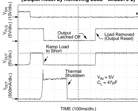
Thermal Shutdown (Output Reset by Removing Load—MIC2076-2)
