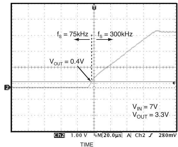
Figure 4. Startup Waveform
