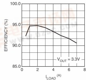
Efficiency for V IN = 5V and V OUT = 3.3V
