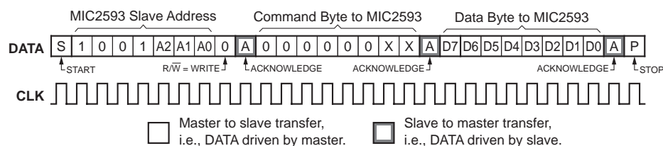
Figure 9. WRITE_BYTE Protocol
