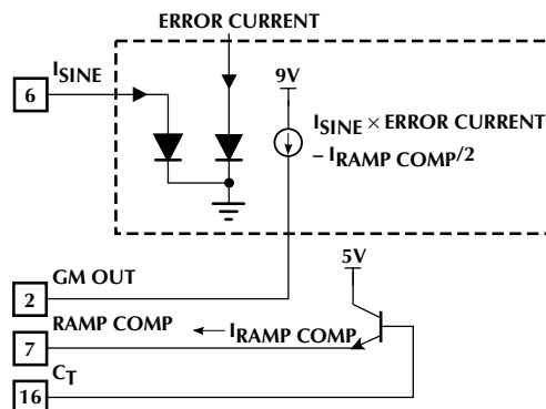
Figure 6. Gain Modulator Block Diagram
