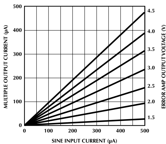
Figure 7. Gain Modulator Linearity
