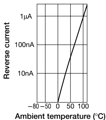
■ Reverse current-Temperature
