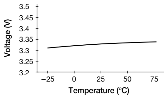
V_{BAT} detection voltage-Temperature
