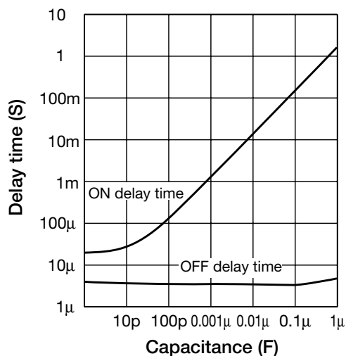
\overline{CS} - \overline{CS} pin ON/OFF delay time vs. capacitance TC
