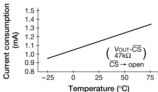
Current consumption-Temperature
