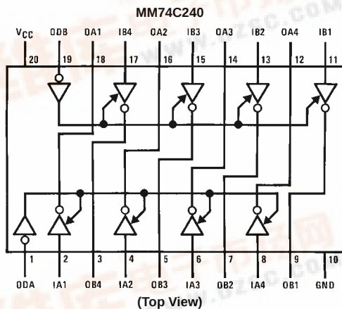
Pin Assignments for DIP and SOIC
