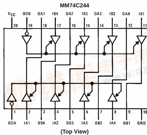
Pin Assignments for DIP and SOIC
