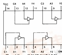
Top View (MM74HC126)
