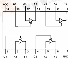
Top View (MM74HC125)
