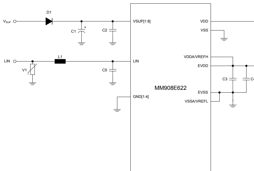
Figure 34. EMC/EMI recommendations
