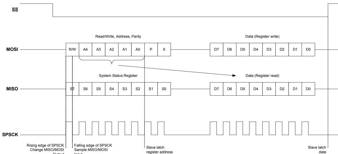
Figure 31. SPI Protocol
