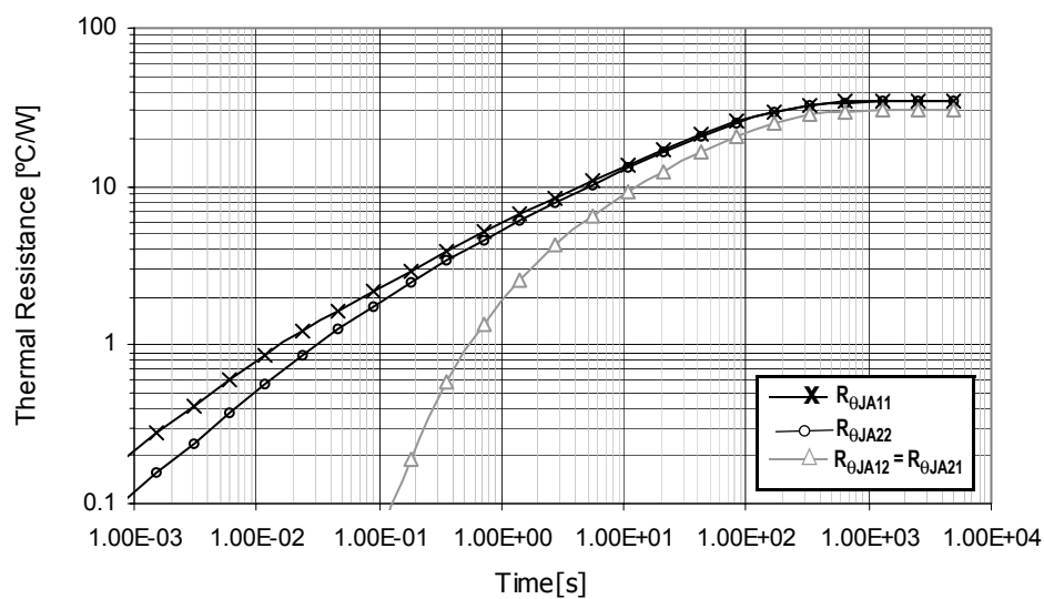
Figure 39. Transient Thermal Resistance R_{\theta JA} (1.0 W Step Response) Device on Thermal Test Board Area A = 600 (mm²)
