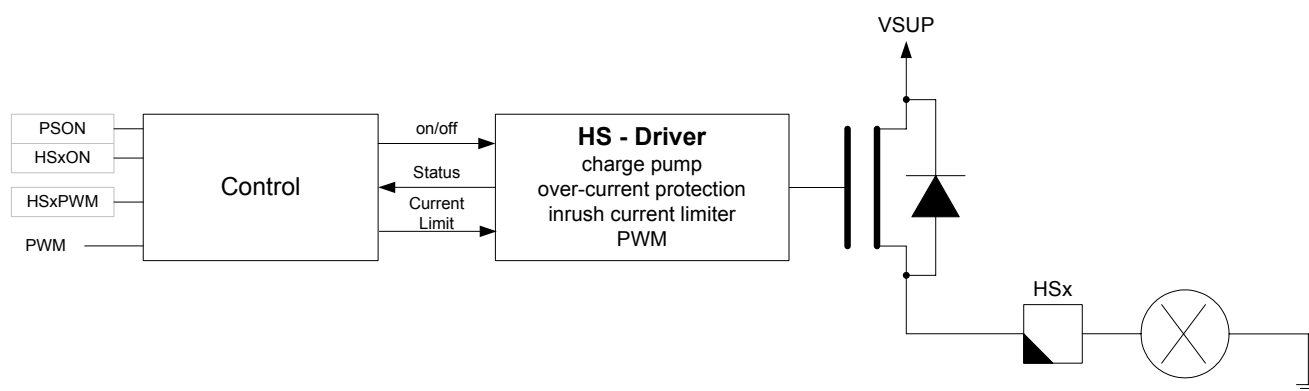
Figure 23. HS circuitry
