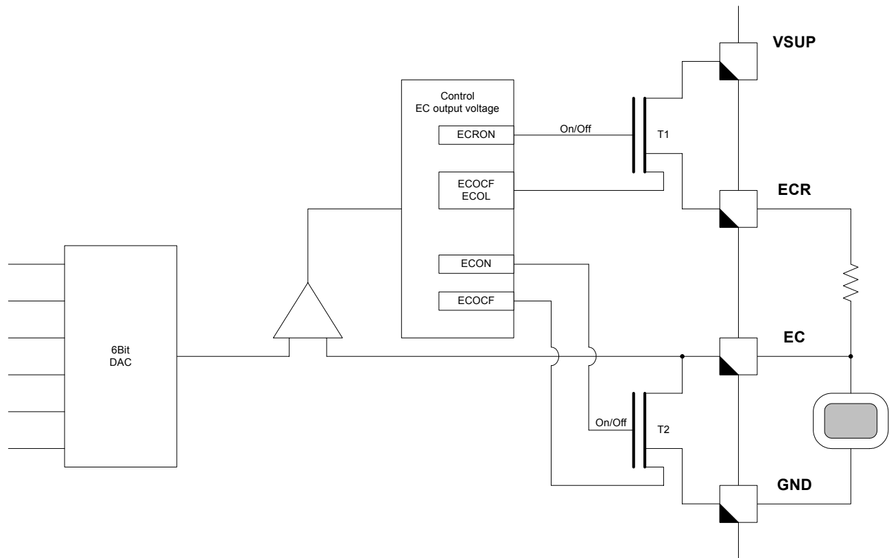
Figure 25. EC Circuitry
