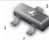
CASE 318, STYLE 6 SOT-23 (TO-236AB)
