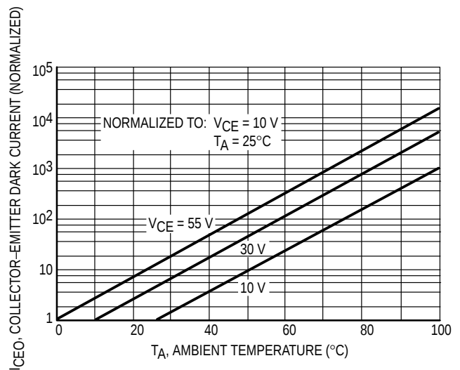
Figure 6. Collector-Emitter Dark Current versus Ambient Temperature
