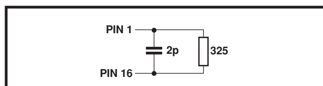
Figure 4 Approximate model of IF output
