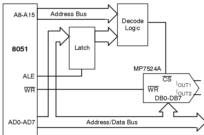
Figure 3. Microcontroller Interface
