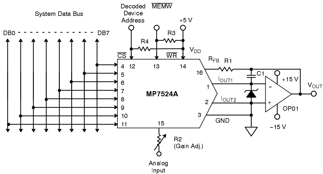
Figure 5. MP7524A/8080A Interface
