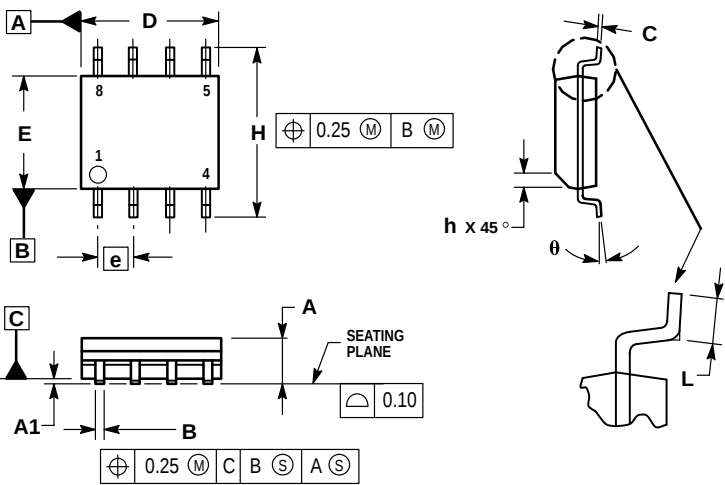
D SUFFIX PLASTIC SOIC PACKAGE CASE 751-05 ISSUE S
