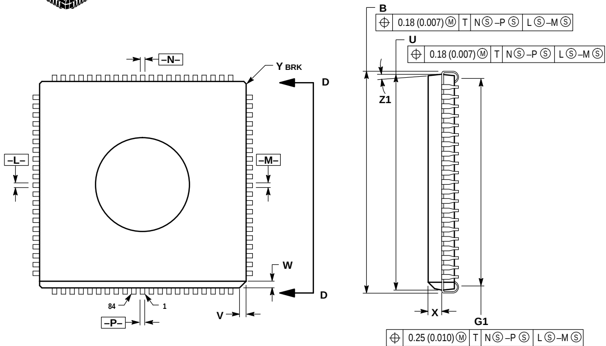
DETAIL D-D
