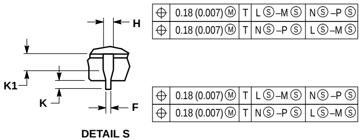
DETAIL S
