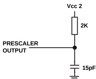
Fig.5 Maximum prescaler output load
