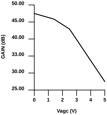
Fig. 6 AGC operation
