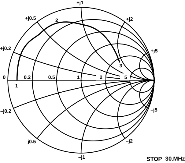
Fig. 8 Output impedance
