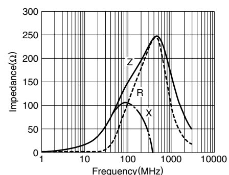
MPZ1608D101B
