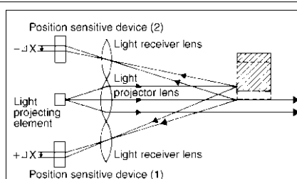
Fig. 2 Triple beam range measurement method By averaging the range measurement signals of the 2 light receiving systems, the range measurement difference is cancelled.
