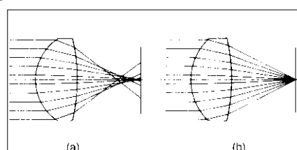
Fig. 3 Light beam trace of the lens (a) is a spherical lens, and (b) is the aspherical lens. Because there is no aberration in (b), range measurement precision is high.
