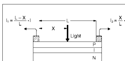
Fig. 4 PSD (position sensitive device) construction By making a calculation of the ratio of I_1 and I_2 , the light spot position can be detected.
