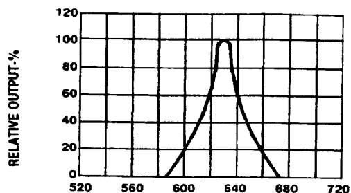
Fig.2 SPECTRAL RESPONSE
