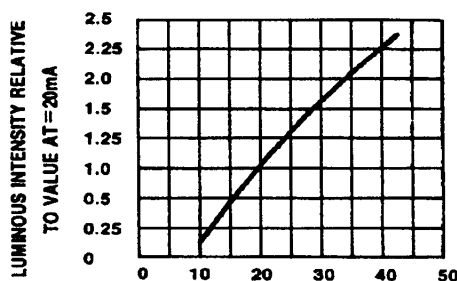
Fig.3 RELATIVE LUMINOUS INTENSITY VS. FORWARD CURRENT
